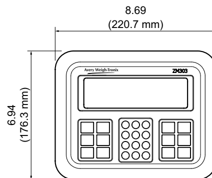
Panel Mount
